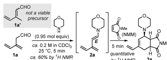
Scheme 2. Generation and Diels–Alder reaction of trienamine 2a .
